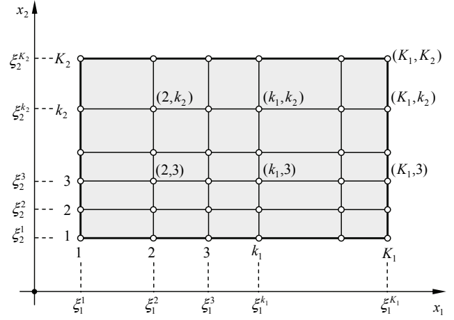
Fig. 1.2. Example of a mesh of sampling points in a 2D domain
